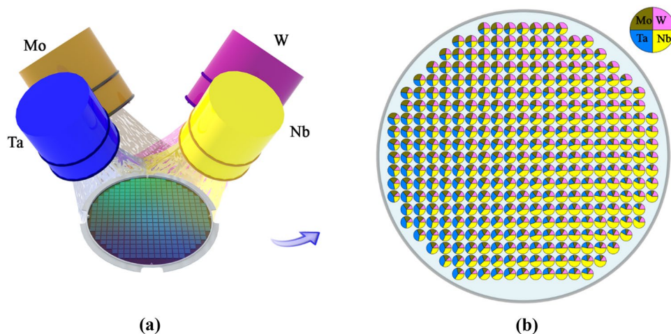
Fig. 1 Schematic visualization of the combinatorial co-sputter process for the synthesis of the quaternary composition spread thin-film MLs. a Confo-cal magnetron sputter cathode arrangement for the co-deposition of Nb–Mo–Ta–W MLs. b Pie chart diagram indicating the relative elemental compositions at each of the 342 MAs. The legend shows the locations of elements
